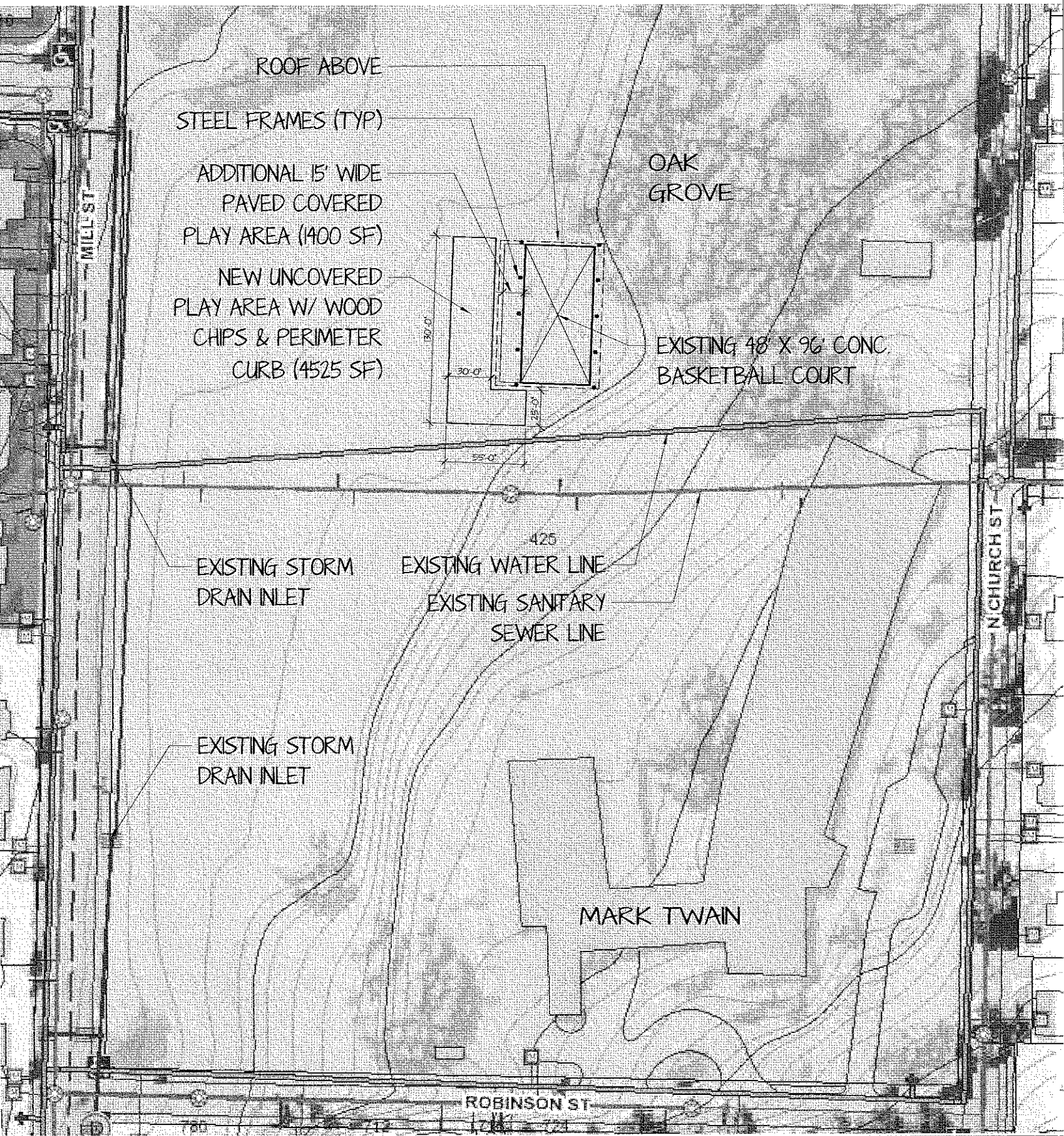
1 SITE PLAN 1"=50'
